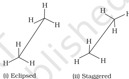
Fig. 13.2 Sawhorse projections of ethane
