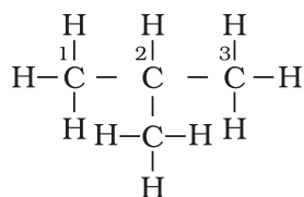
2-Methylpropane (isobutane) (b.p. 261 K)
