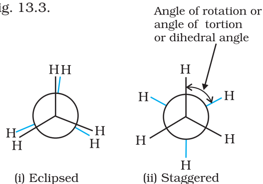
Fig. 13.3 Newman's projections of ethane
