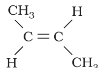
trans -But-2-ene (b.p. 274 K)
