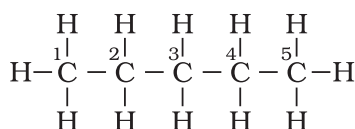
Pentane ( n -pentane) (b.p. 309 K)
