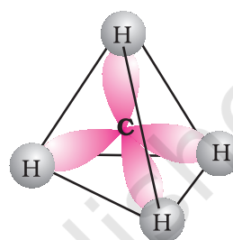
Fig. 13.1 Structure of methane
