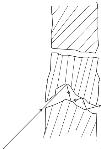
Fig. 13.5 Molecules going through a porous wall.
