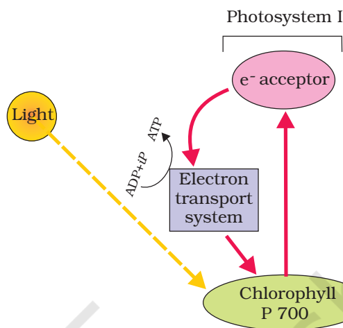
Figure 13.6 Cyclic photophosphorylation
