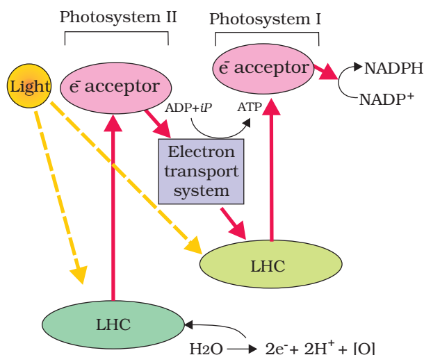
Figure 13.5 Z scheme of light reaction
