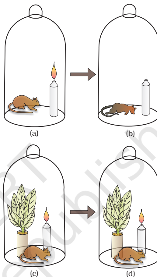
Figure 13.1 Priestley's experiment
