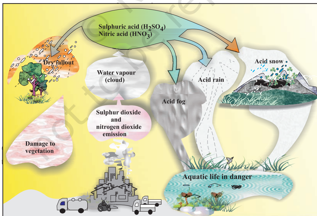
Fig. 14.1 Acid deposition
