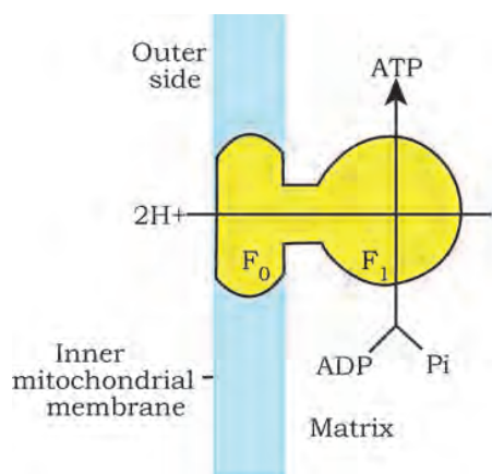
Figure 14.5 Diagrammatic presentation of ATP synthesis in mitochondria
