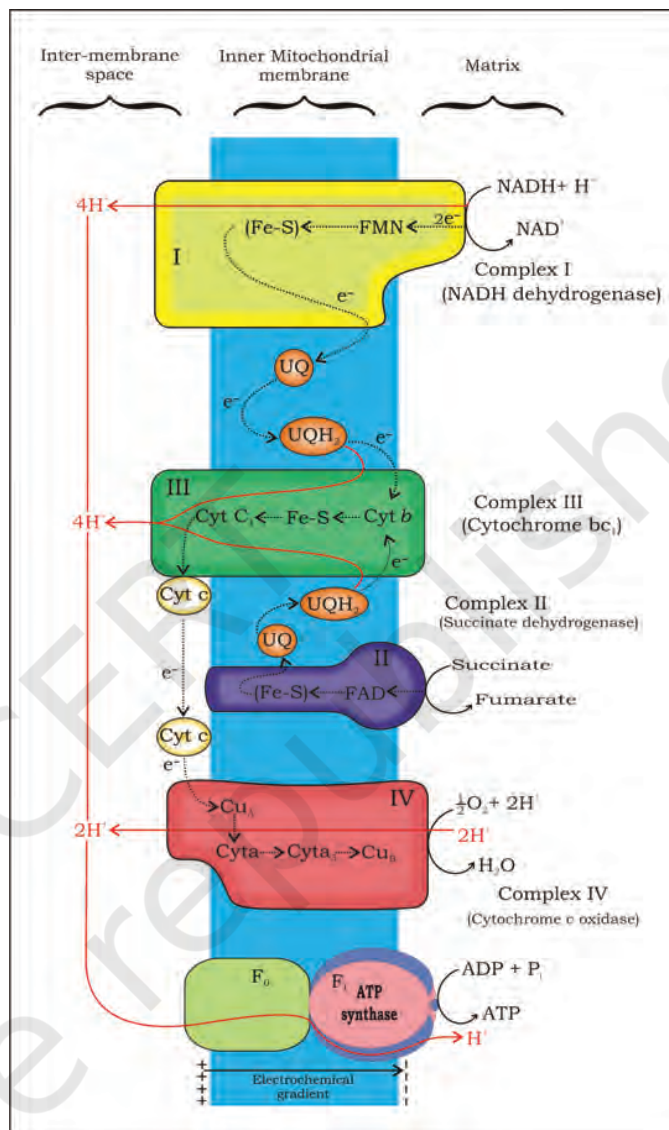
Figure 14.4 Electron Transport System (ETS)
