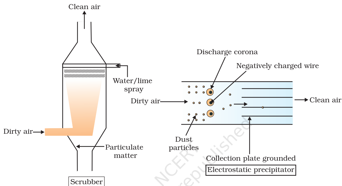
Figure 16.1 Electrostatic precipitator
