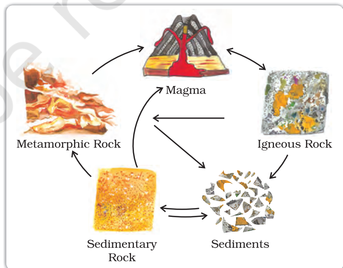
Fig. 2.4: Rock Cycle
