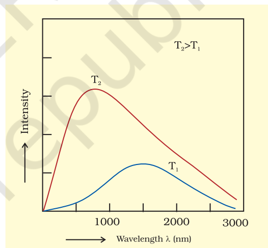
Fig. 2.8 Wavelength-intensity relationship
