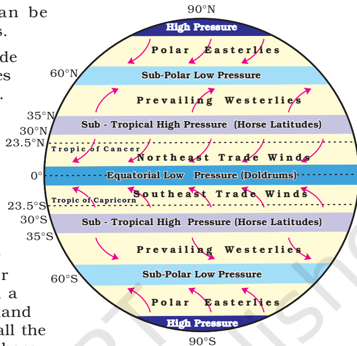
Fig. 4.4: Major Pressure Belts and Wind System
