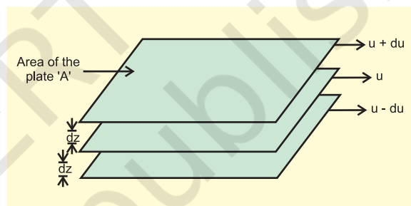
Fig. 5.16 Gradation of velocity in the laminar flow
