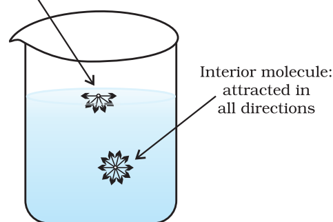
Fig. 5.15 Forces acting on a molecule on liquid surface and on a molecule inside the liquid
