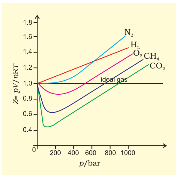
Fig. 5.12 Variation of compressibility factor for some gases
