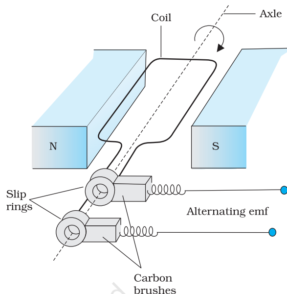
FIGURE 6.16 AC Generator
