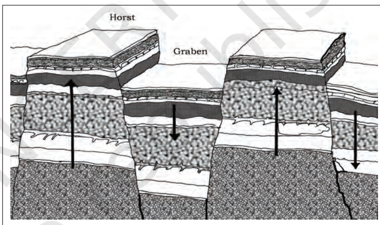
Figure 6.3 : A Block Mountain
