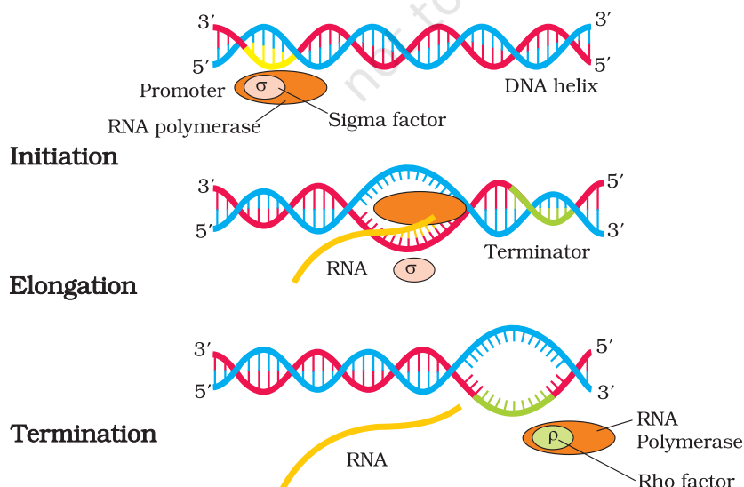
Figure 6.10 Process of Transcription in Bacteria
