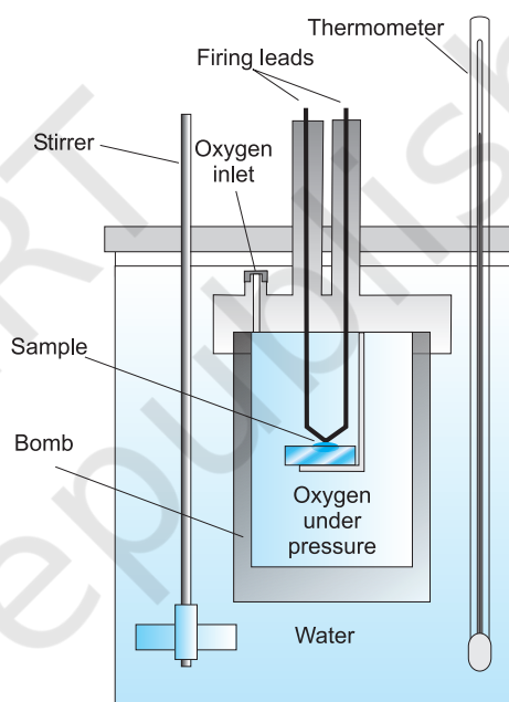
Fig. 6.7 Bomb calorimeter
