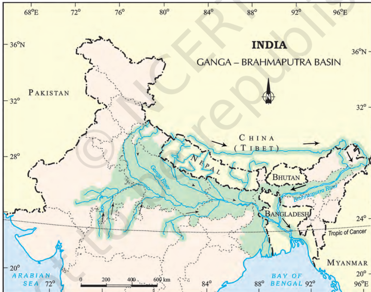
Fig. 8.8: Ganga-Brahmaputra Basin
