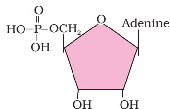
Adenylic acid
