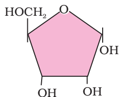
C_5H_{10}O_5 (Ribose)
