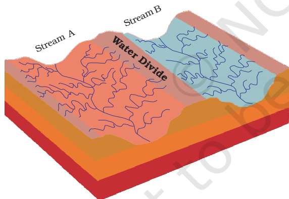
Figure 3.1 : Water Divide
