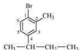
1-Bromo-4-sec-butyl-2-methylbenzene
