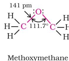
Fig. 11.1: Structures of methanol, phenol and methoxymethane
