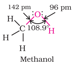
Fig. 11.1: Structures of methanol, phenol and methoxymethane
