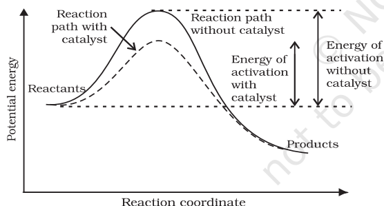
Fig. 4.11: Effect of catalyst on activation energy
