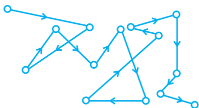
Fig. 5.12: Brownian movement
