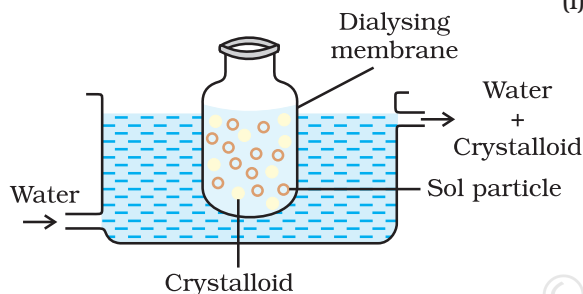
Fig. 5.9: Dialysis
