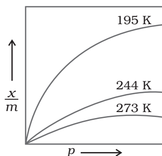
Fig. 5.1: Adsorption isotherm
