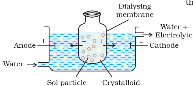
Fig. 5.10: Electro-dialysis
