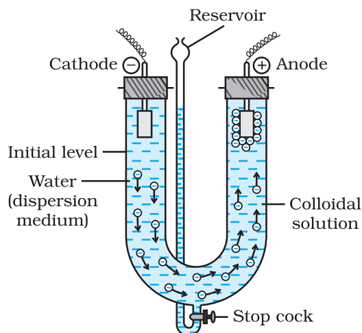
Fig. 5.14: Electrophoresis
