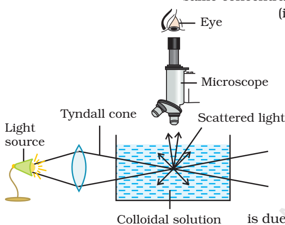
Fig. 5.11: Tyndall effect
