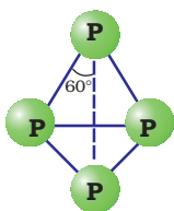
Fig. 7.2 White phosphorus
