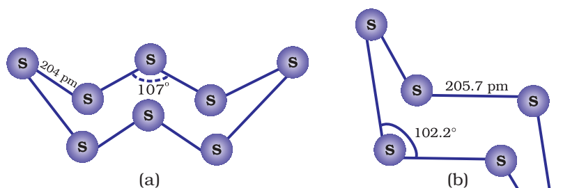
Fig. 7.5: The structures of (a) S_8 ring in rhombic sulphur and (b) S_6 form
