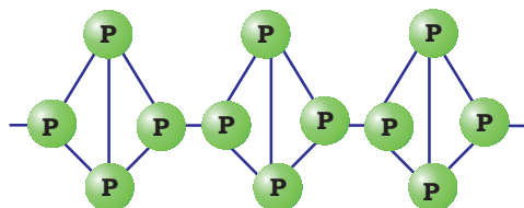
Fig.7.3: Red phosphorus
