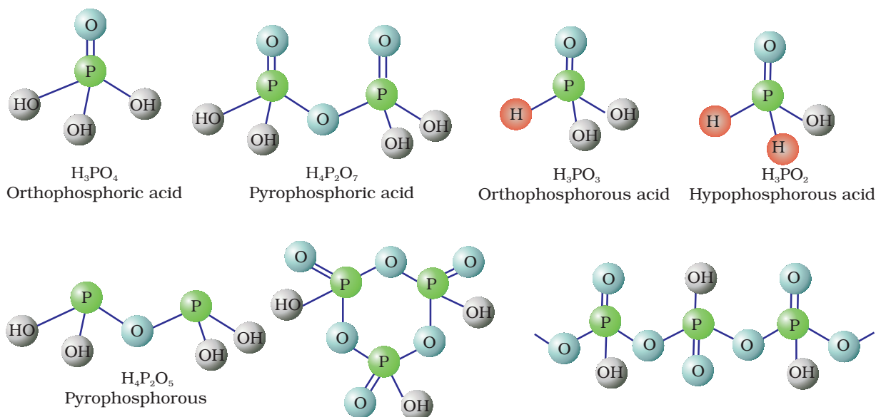
Fig. 7.4 Structures of some important oxoacids of phosphorus
