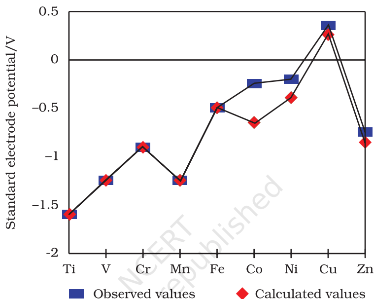
Fig. 8.4: Observed and calculated values for the standard electrode potentials ( M^{2+} \rightarrow M^\circ ) of the elements Ti to Zn
