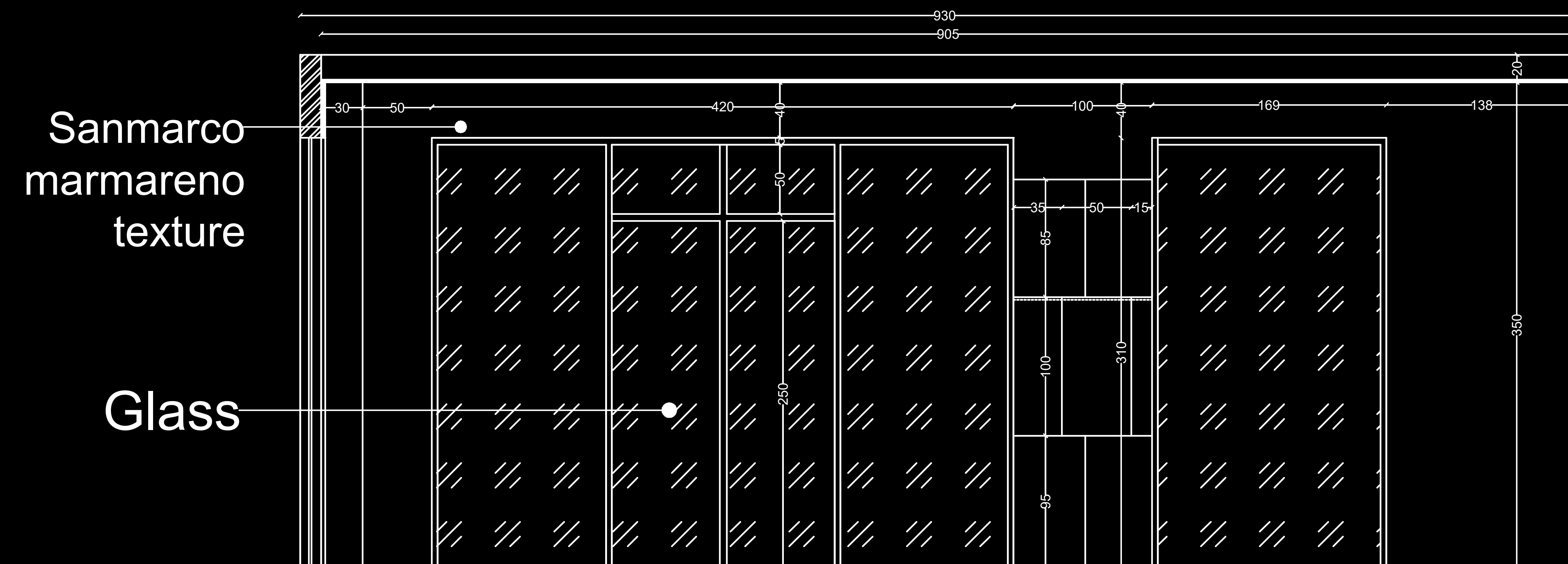
Sec B-B
