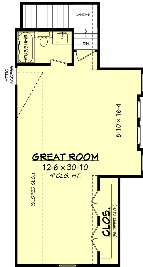
BONUS FLOOR PLAN
