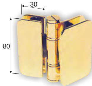
GTR-02 Glas an Glas, 180°
