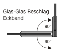
SDH090 Glas an Glas, 90°
