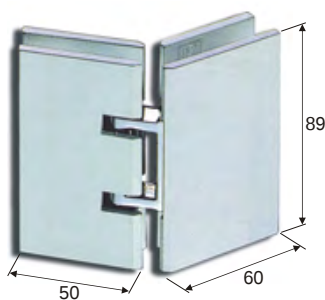
SDH135 Glas an Glas, 135°
