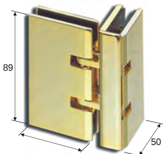
SDH090 Glas an Glas, 90°
