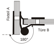
GTR-06 Glas an Glas
