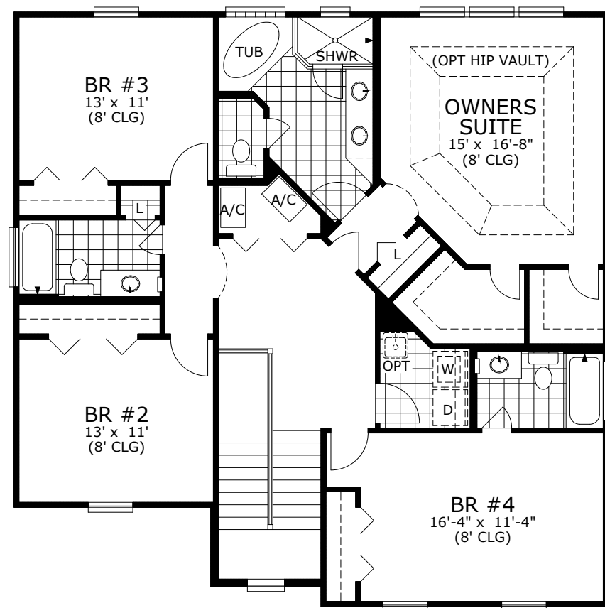
SECOND FLOOR
