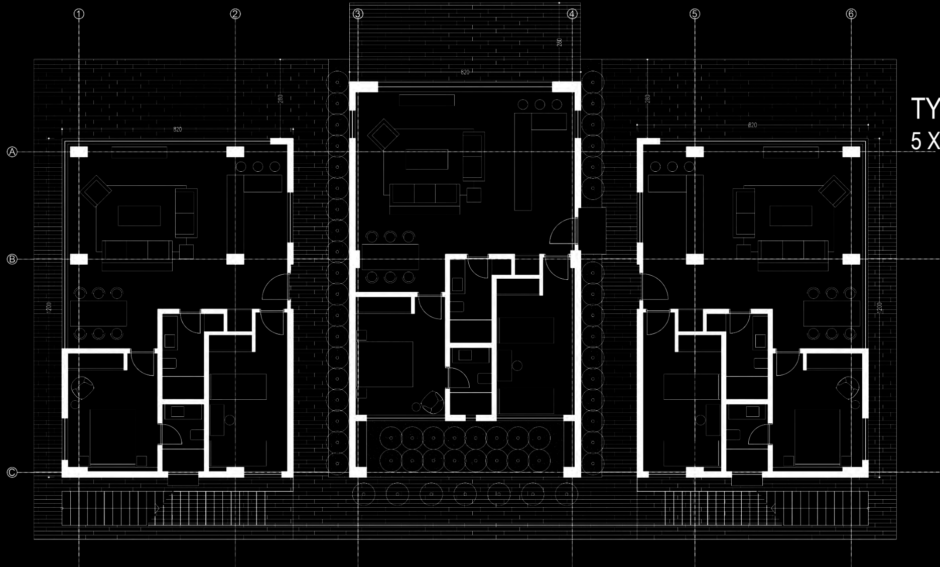
TYPE II GROUND FLOOR PLAN
