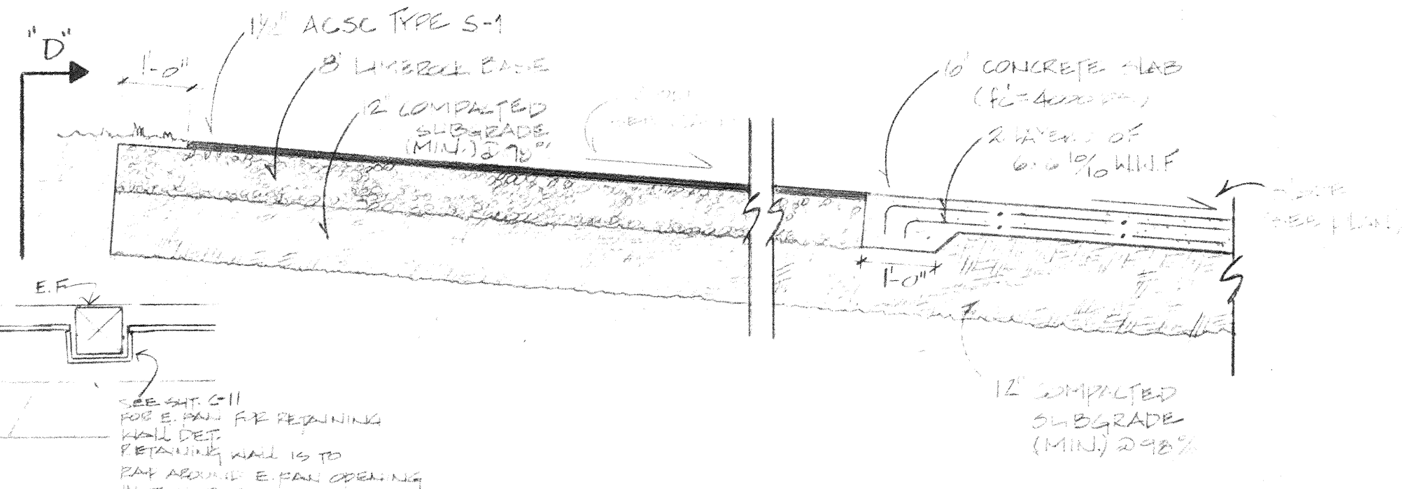
TYPICAL ASPHALT & CONCRETE PAVEMENT SECTIONS H.T.S
