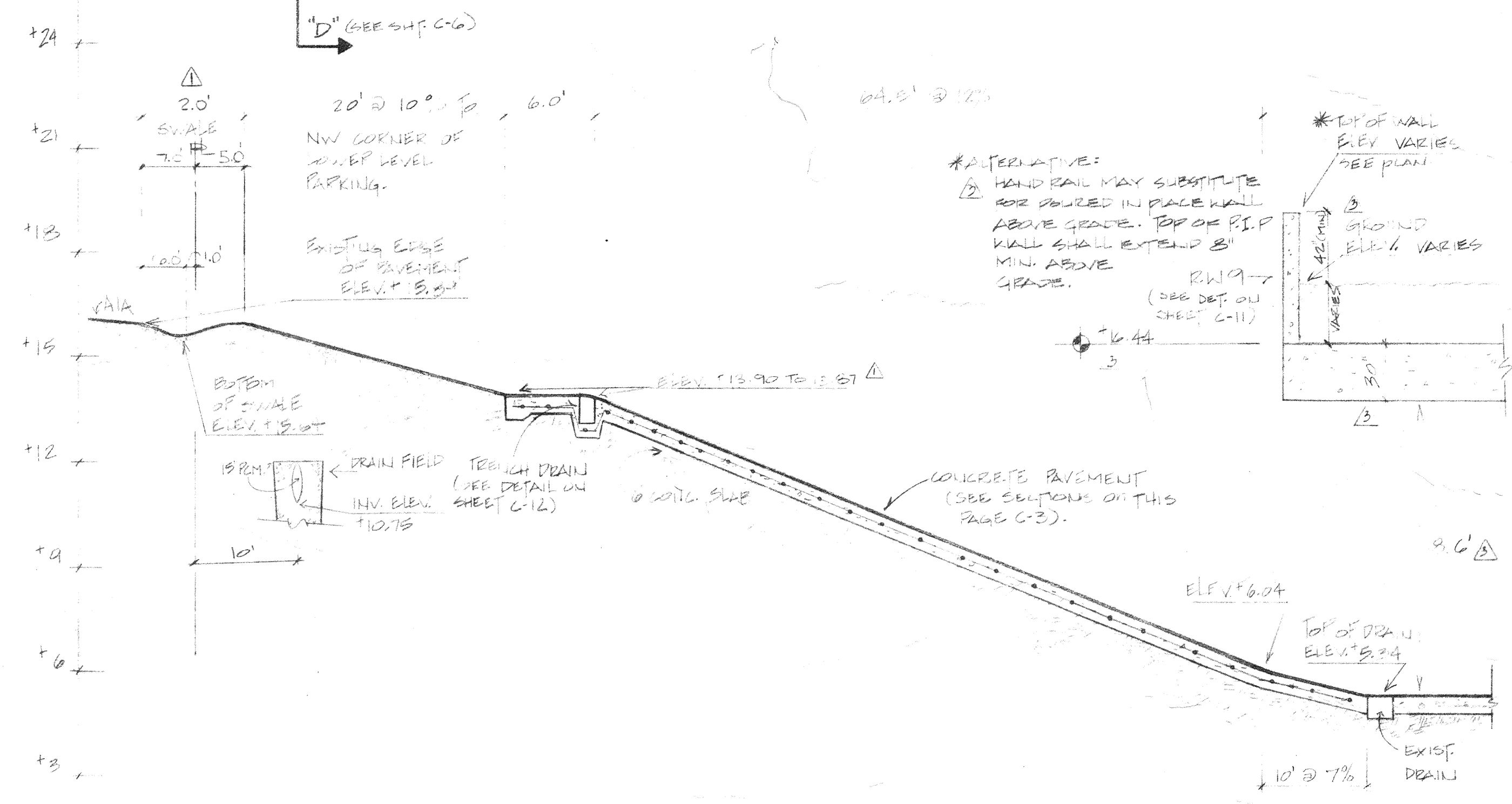
LOWER LEVEL DRIVEWAY (SECTION I-I) SCALE: VERTICAL 1\"/>
