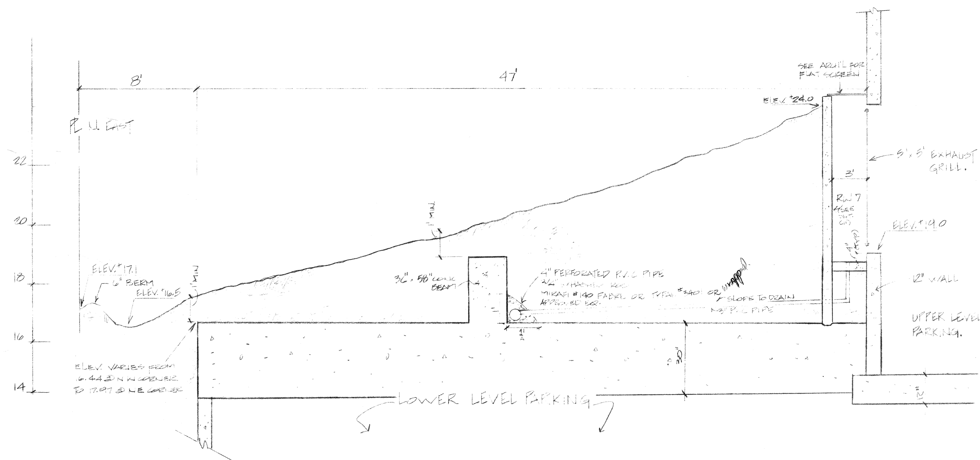
SECTION E-E SCALE: VERTICAL 1" = 2.0' HORIZONTAL 1" = 4.0'
