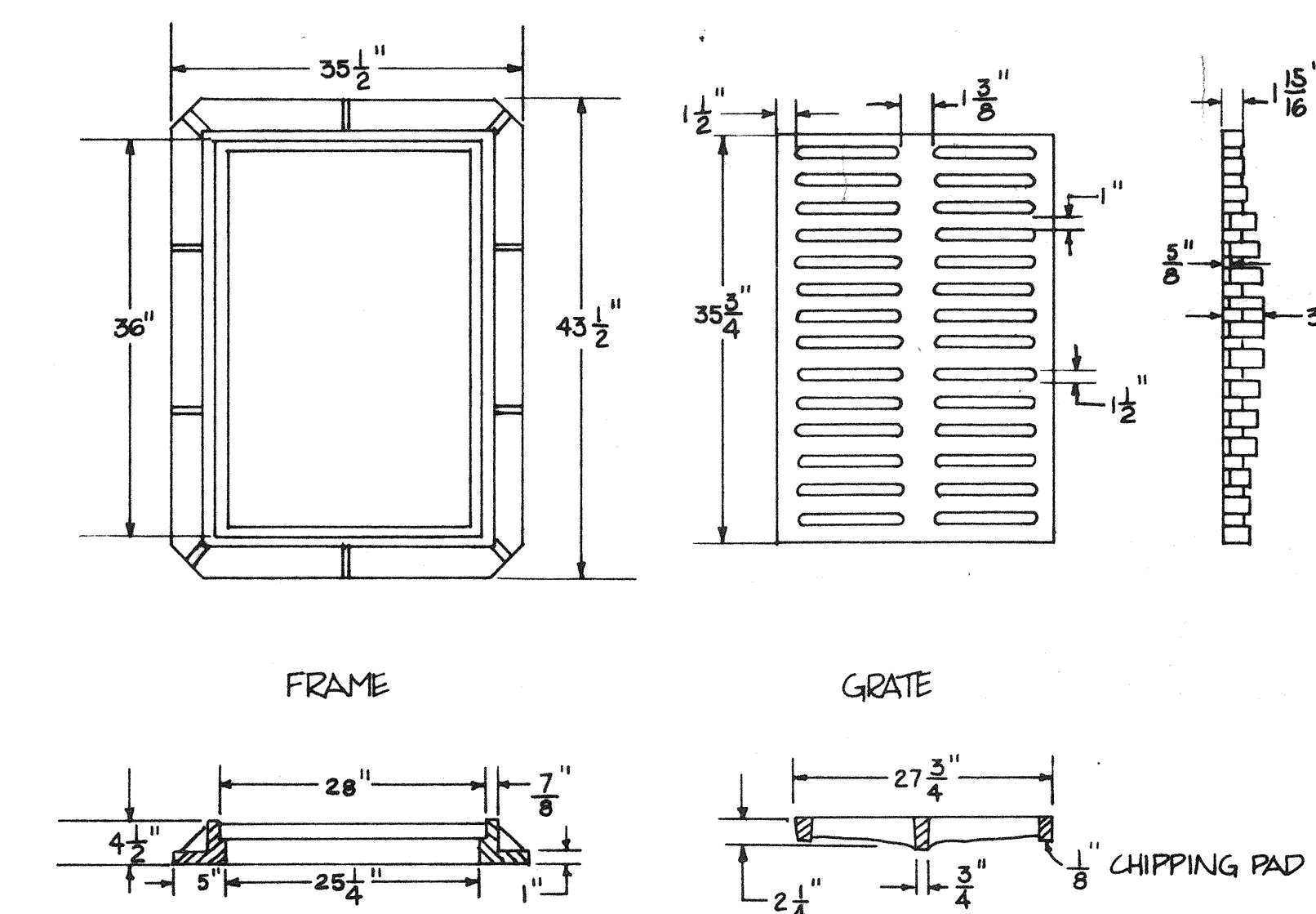
CATCH BASIN FRAME AND GRATE
