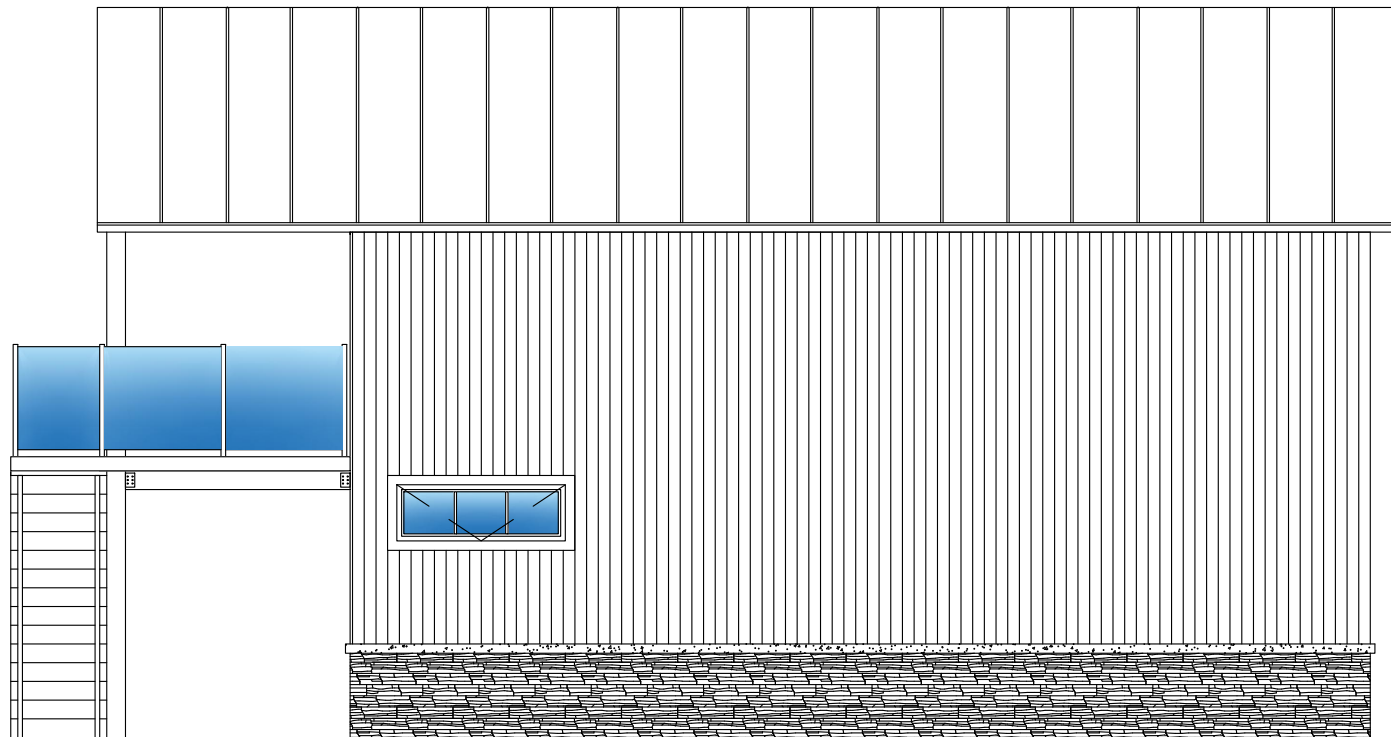
LEFT ELEVATION
