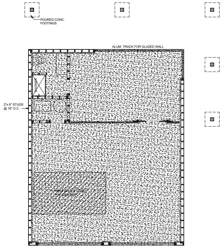
FRAMING PLAN
