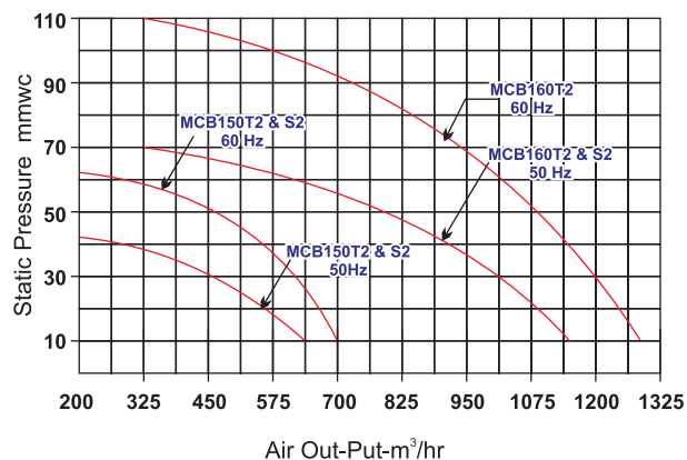
Air Out-Put Vs Static Pressure
