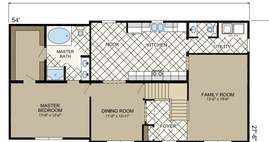
FIRST FLOOR
