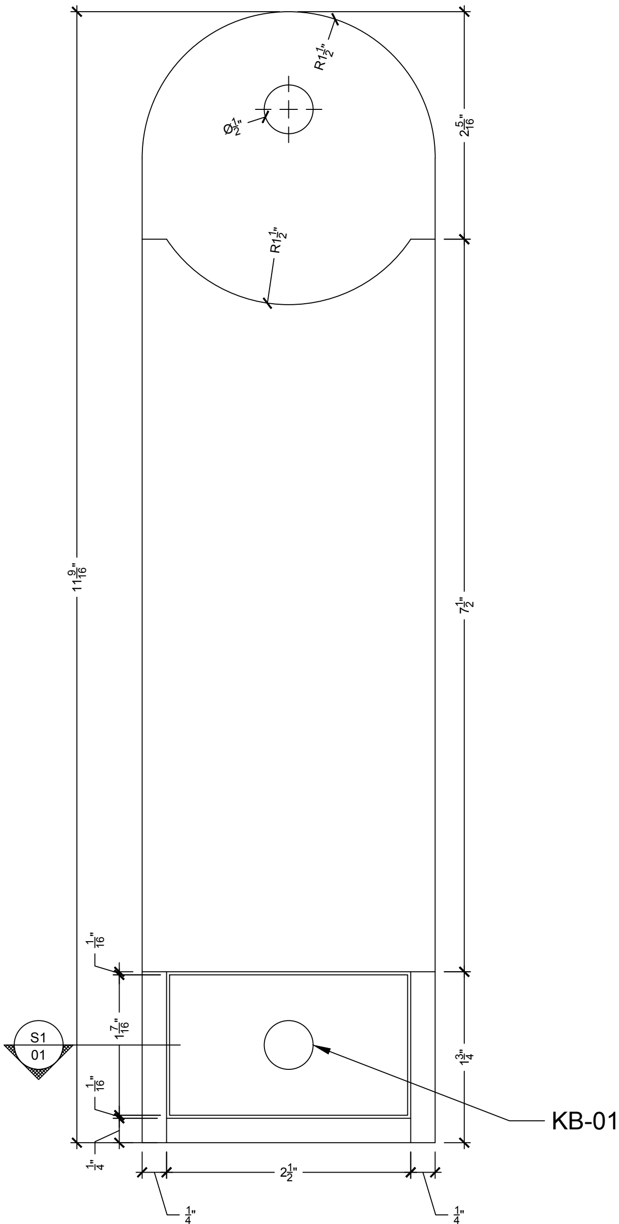
E1 01 ELEVATION: SHAKER CANDLE BOX SCALE: 12" = 1'-0"
