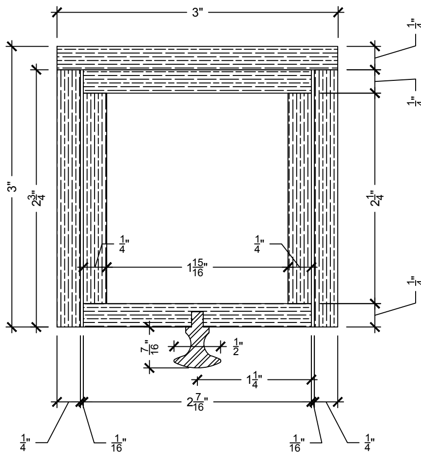
S1 01 SECTION: SHAKER CANDLE BOX SCALE: 12" = 1'-0"
