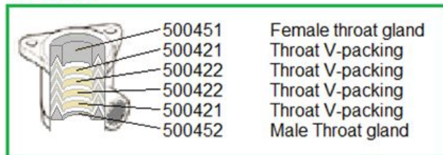
DETAIL 1
