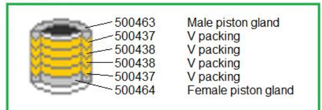
DETAIL 2
