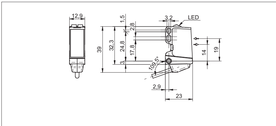
dimension drawing
