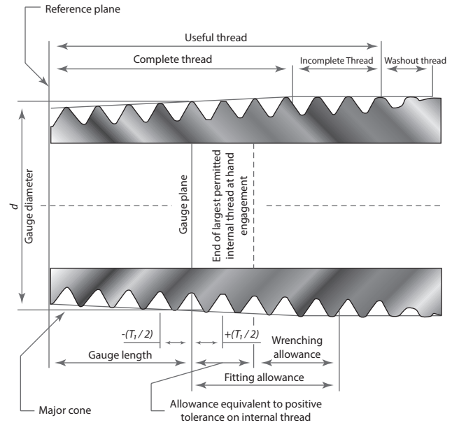
Terms relating to external threads
