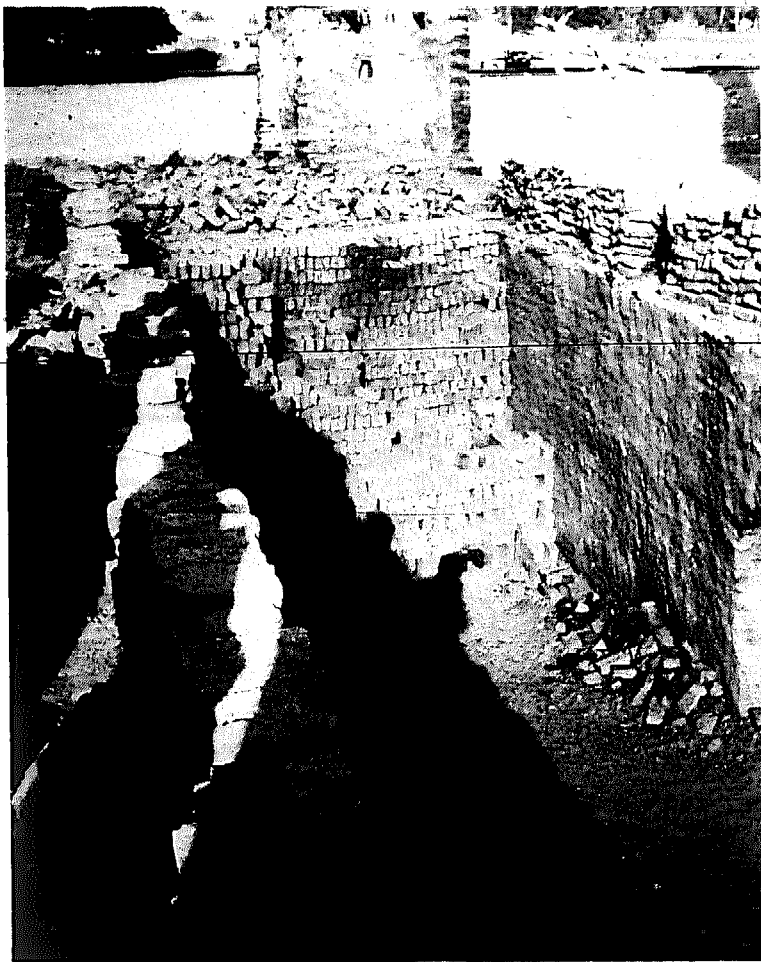
Bricks placed in open setting in deep chamber of continuously firing kiln (fire holes round in a circuit).
