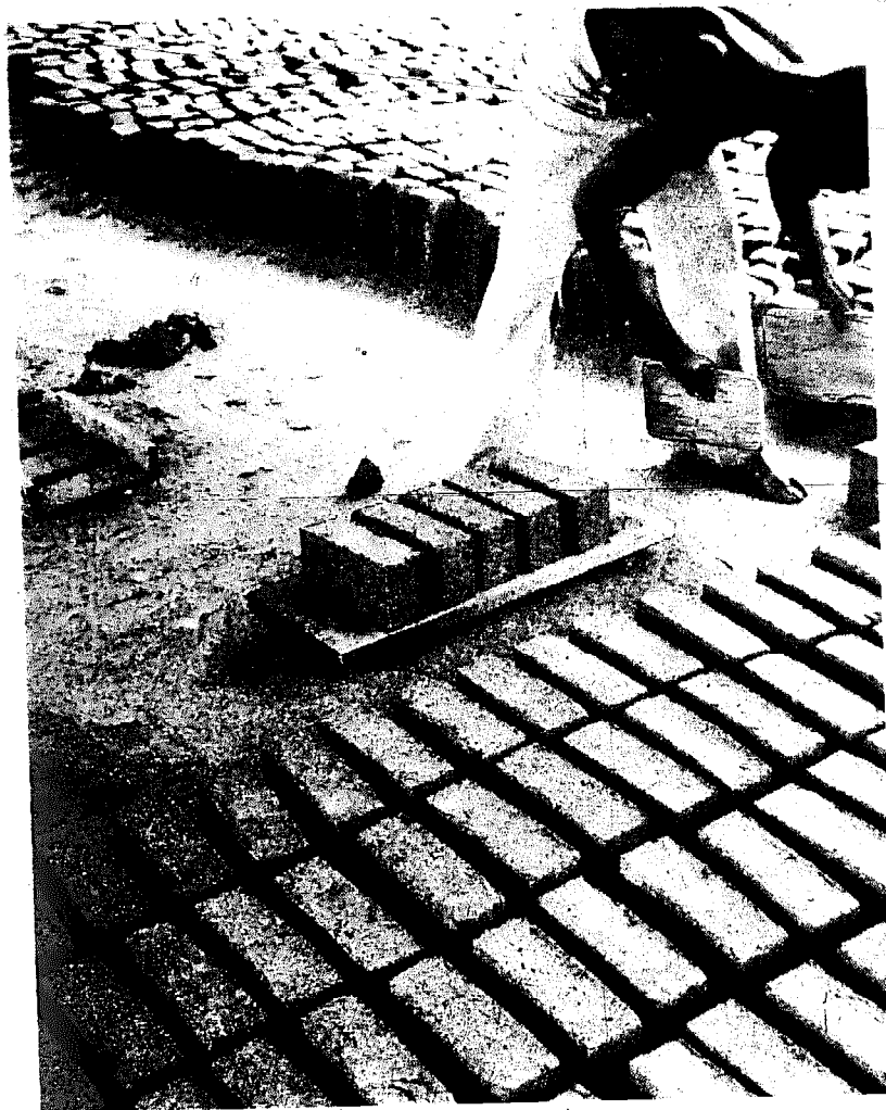
Accurately sandmoulded bricks set out for initial drying. In the background, bricks are upturned to avoid drying distortion
