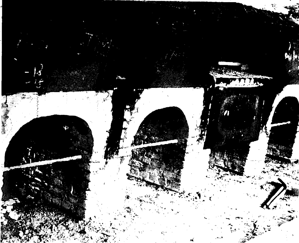
Woodfired kiln in Ghana showing steel plates used to restrict some of the ingress of excess air. Metal grate originally installed has since been removed to ease stoking with long pieces of wood
