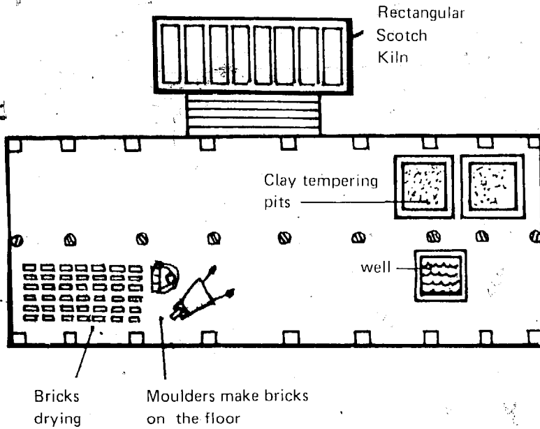
Brickworks layout
