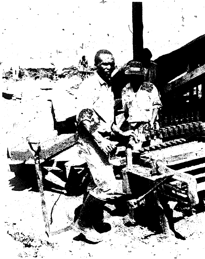
Side cutter producing wirecut bricks from an extruded column, installation partially in the open
