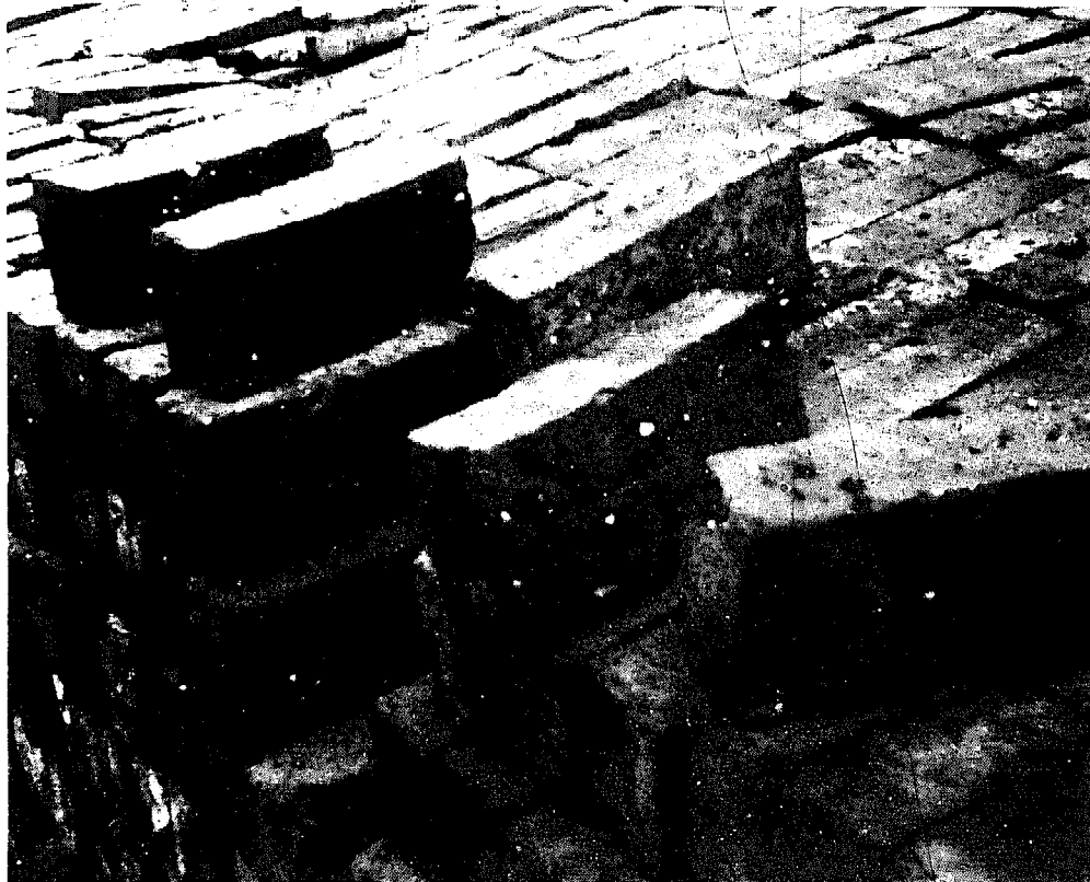
Addition of coal or clinker lumps to the clay may harm the appearance and strength of the finished bricks if the lumps are too big and create intrusions of ash. This process would be made acceptable if a simple grinding system were available to reduce the particle size
