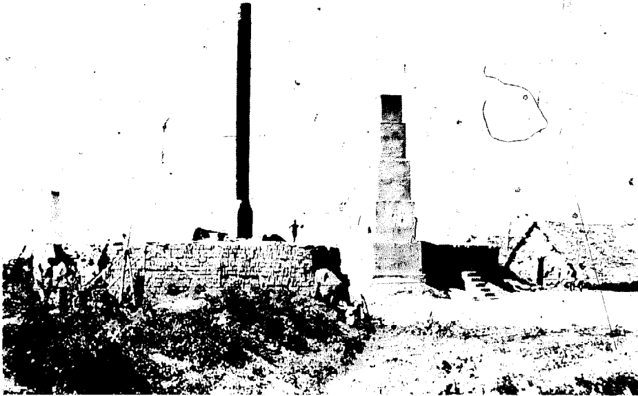
General view of plant showing movable metal chimney alongside permanent brick chimney. Note covered production building on right side of picture
