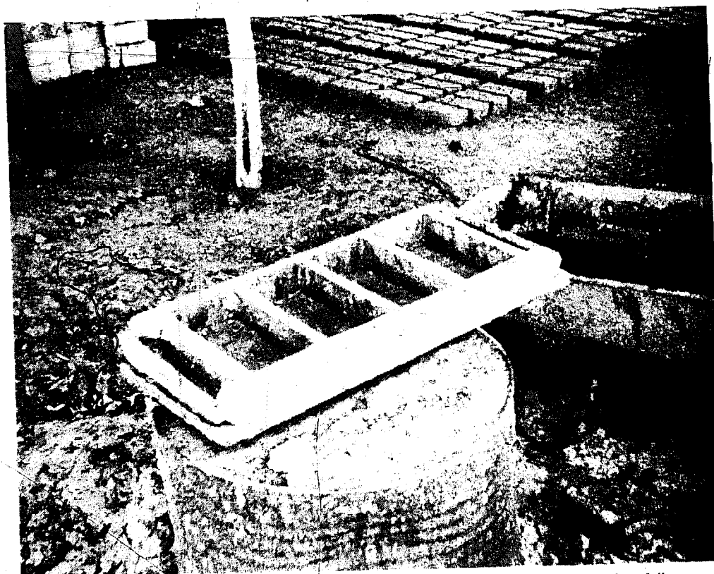
Four-compartment slop mould – an unsuccessful technical innovation being over 20 kg when full and difficult to handle
