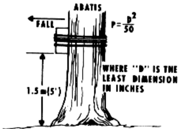
Figure 4 Charge Placement
