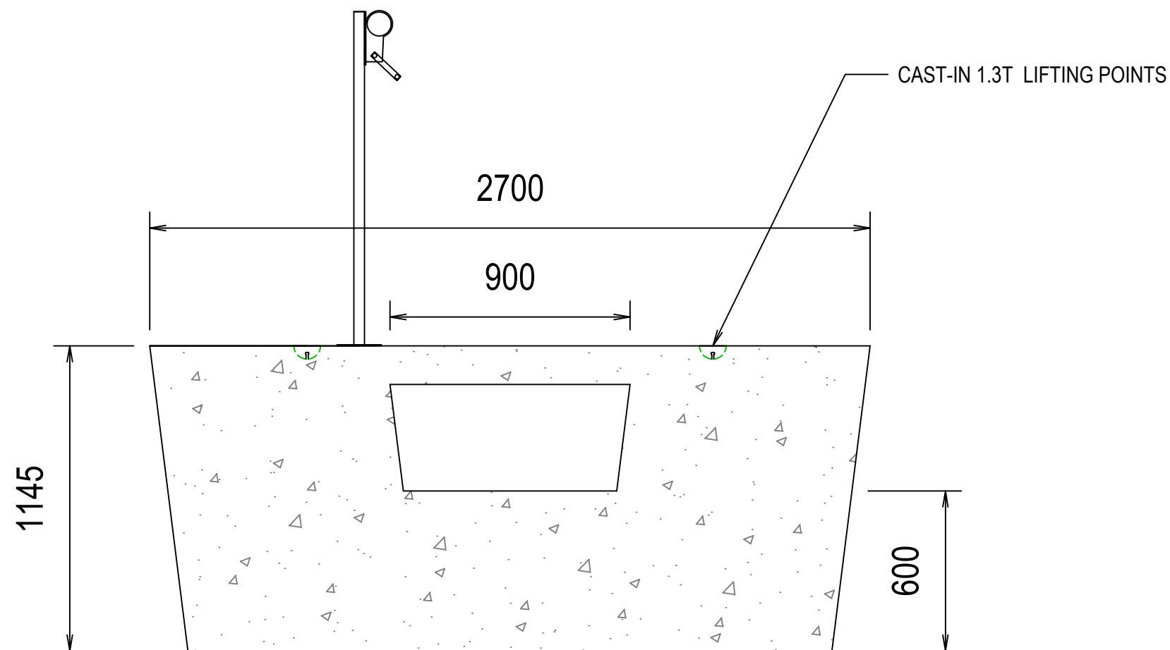
T3 - 900×400 OPENING
