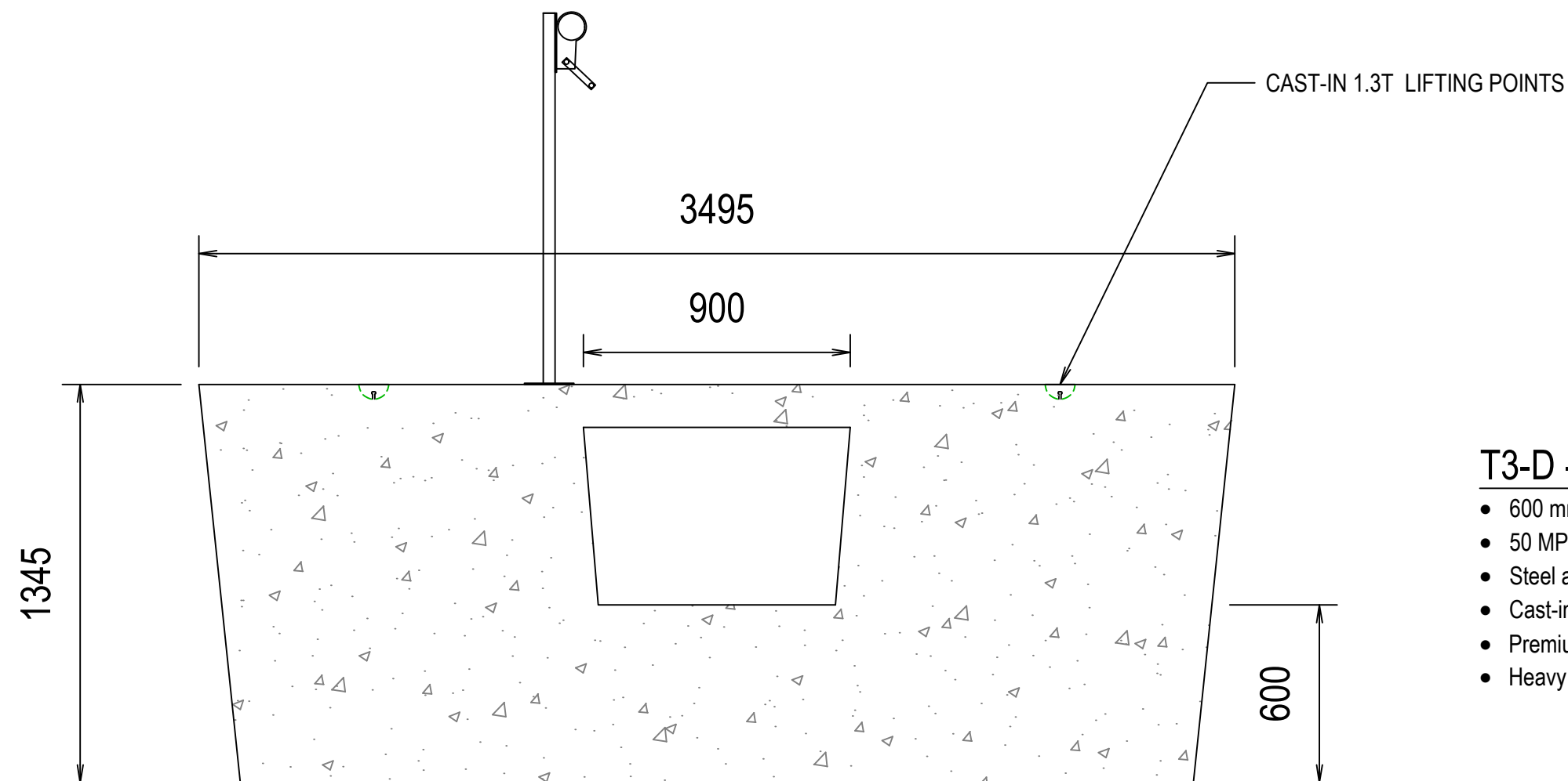
T3-D - 900×600 OPENING
