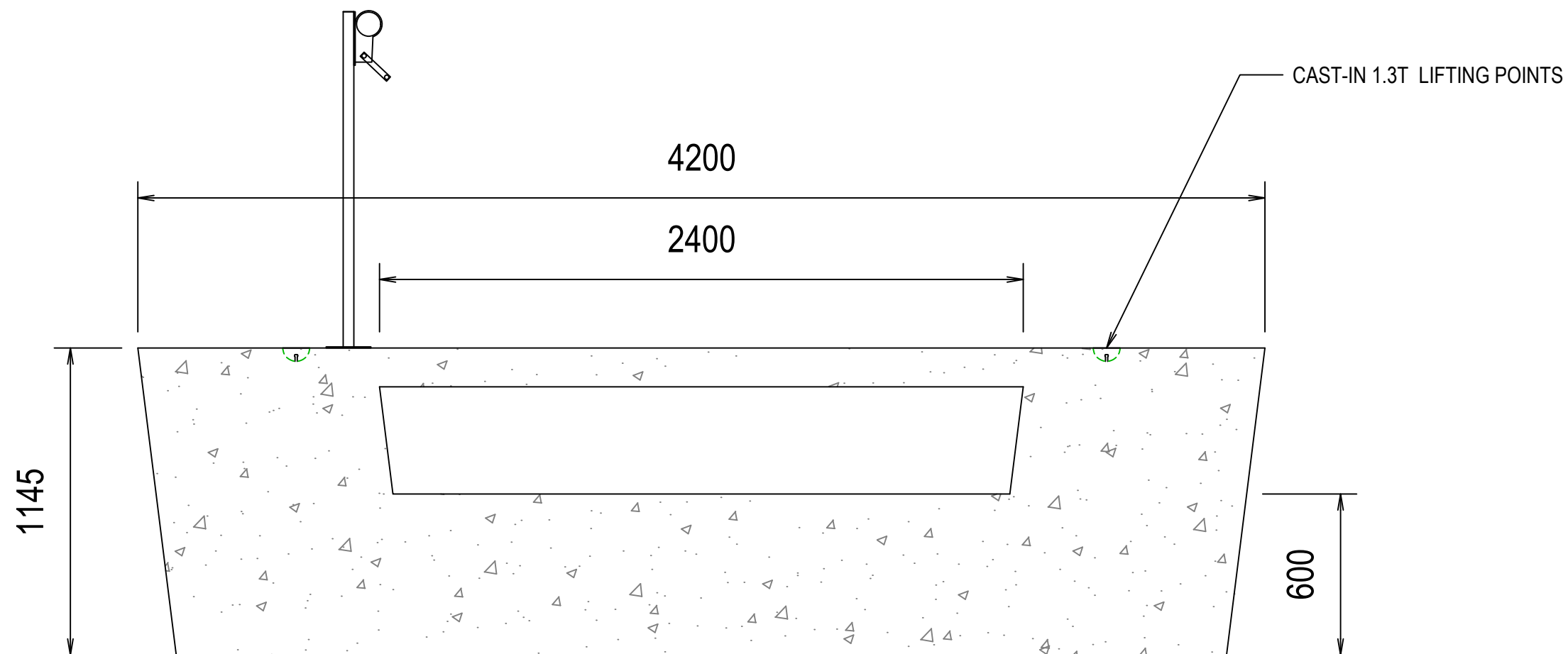
T8 - 2400×400 OPENING
