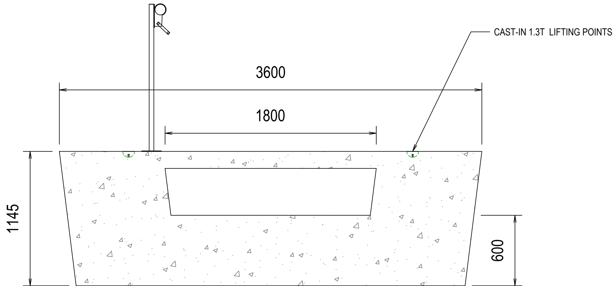
T6 - 1800×400 OPENING
