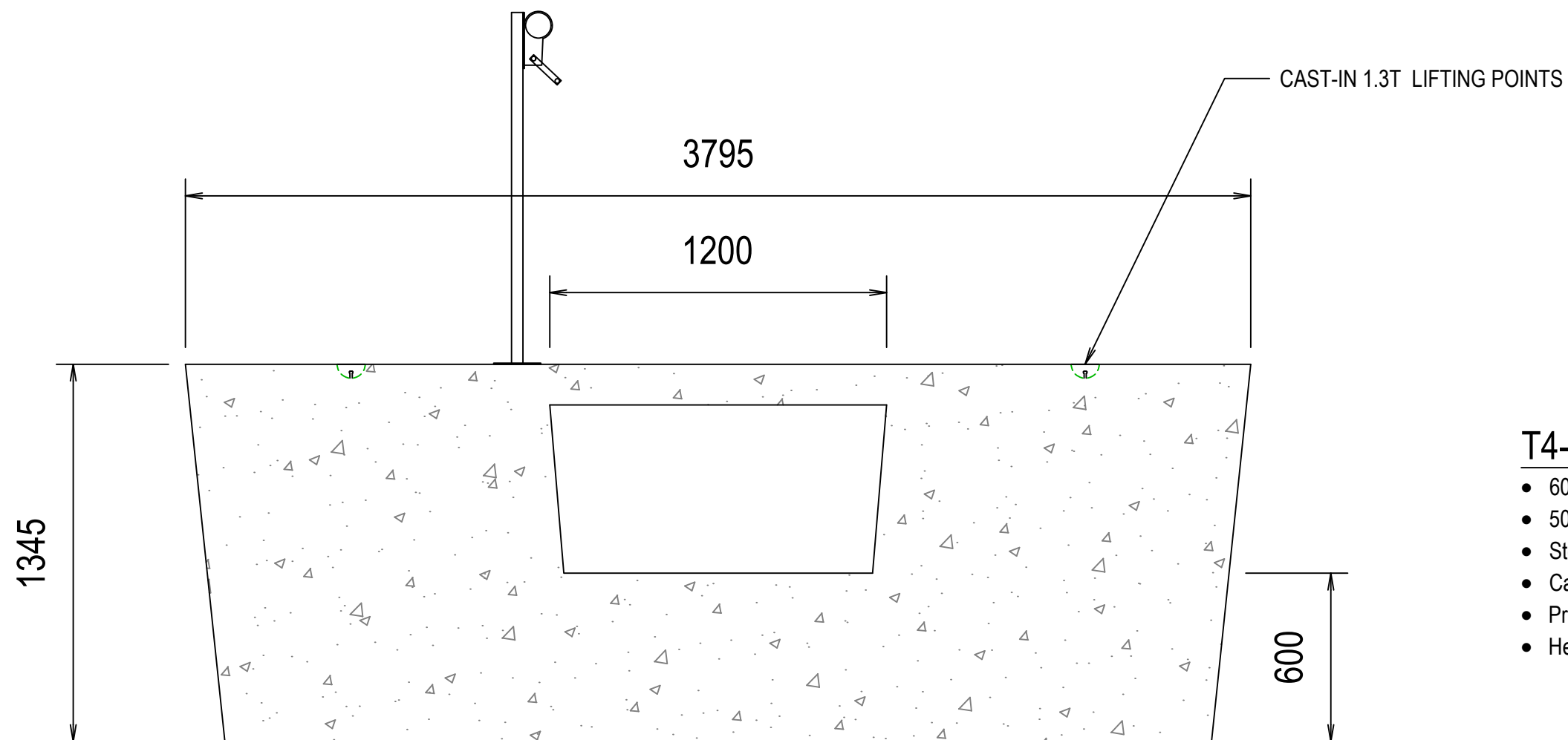
T4-D - 1200×600 OPENING
