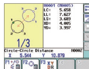
KA 200 Counter
