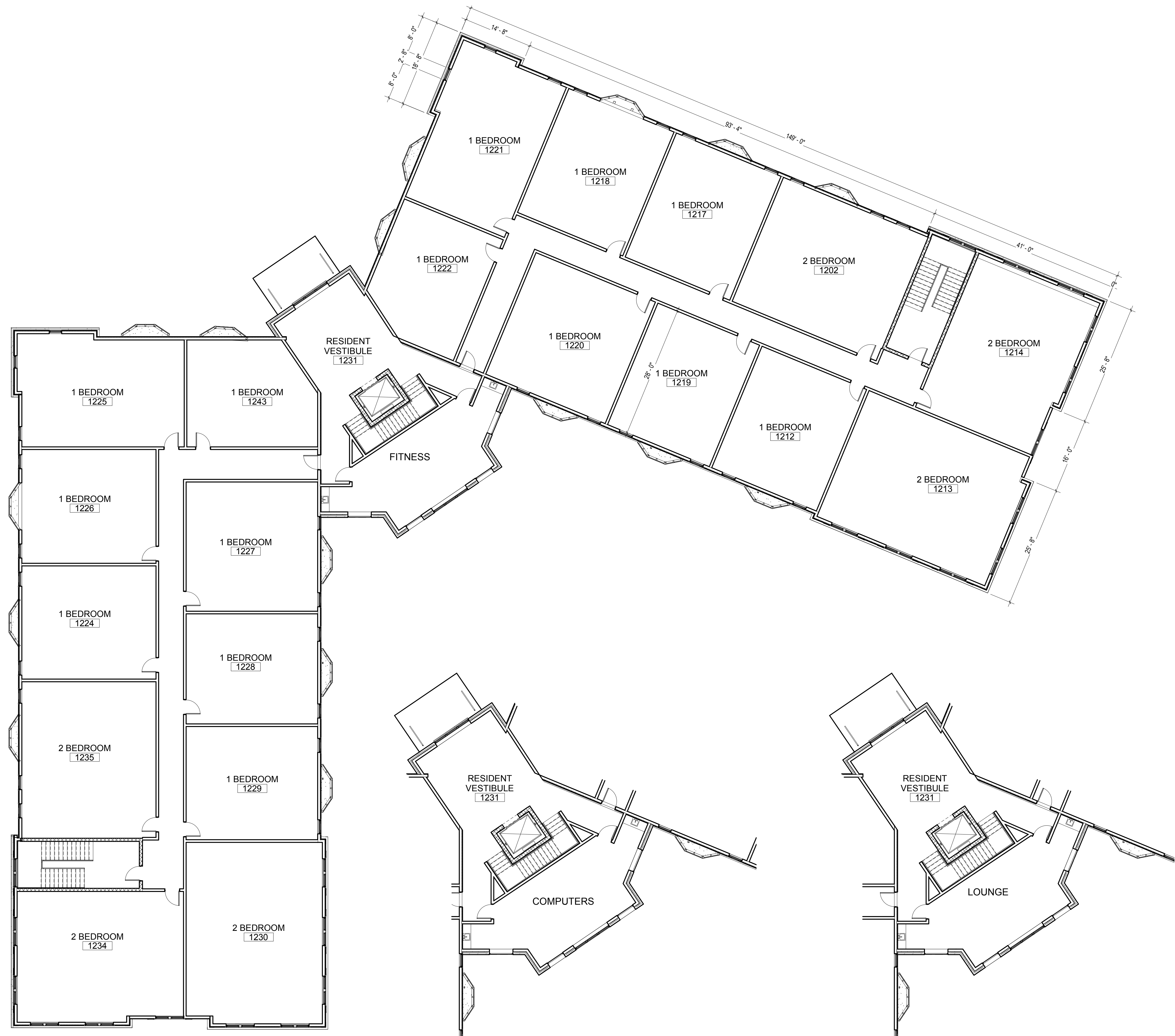
BUILDING D- SECOND, THIRD & FOURTH FLOOR PLAN
