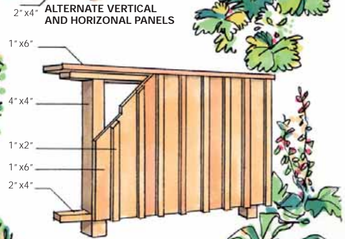
VERTICAL BOARD-AND-BATTEN
