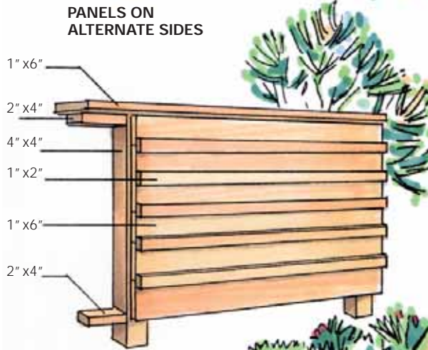
HORIZONTAL BOARD-AND-BATTEN
