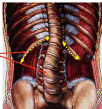
Fig. 5 Our hypothesis on the increased relative length of the 12th rib on the convexity of right lumbar idiopathic scoliotic curves
