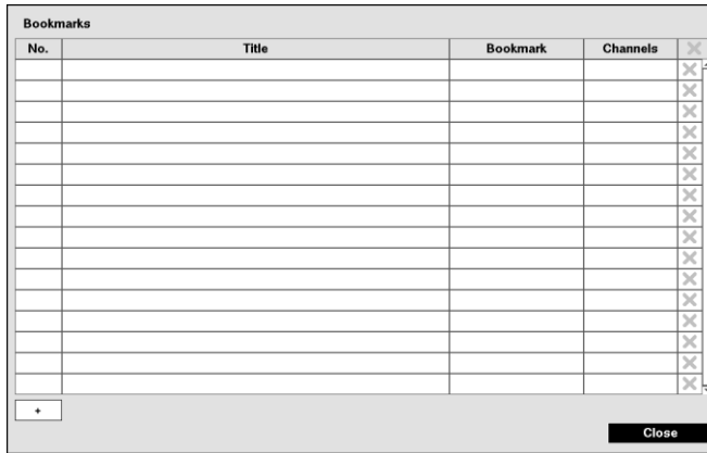
Figure 56: Bookmarks screen.
