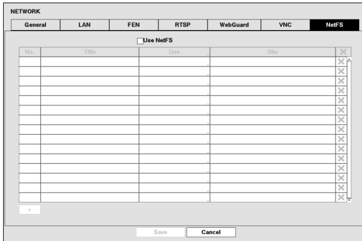
Figure 36: Network – NetFS.
