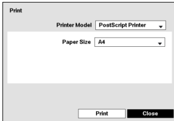
Figure 58: Print screen.
