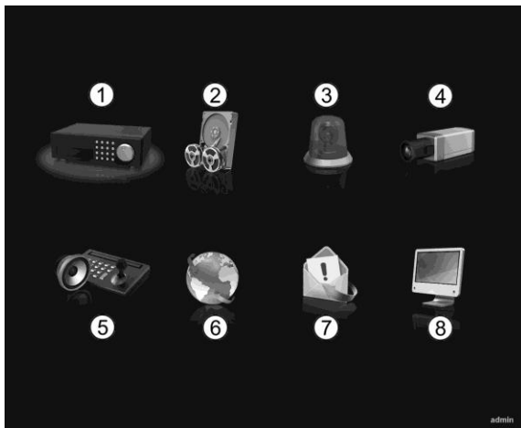
Figure 4: Setup screen.
